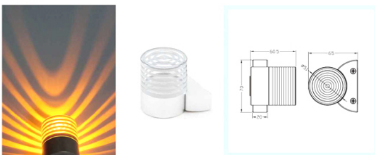
MS-WL51B
